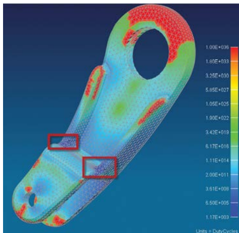
Durability results based on a flexible body motion simulation of motorcycle suspension bracket.
