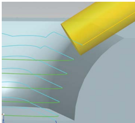
5-axis flank milling options make smaller cusps.
