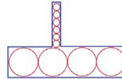
Illustration of “rolling ball” algorithm where the software uses the diameter of a ball at a given location as the thickness of the part at that location.
