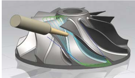
New finish patterns allow incremental finishing for thin blades.
