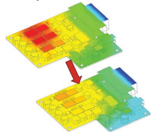
Minimizing critical component temperature by optimizing flowrate.
