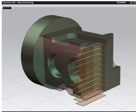
Volume-based 2.5D milling speeds programming for machinery.
