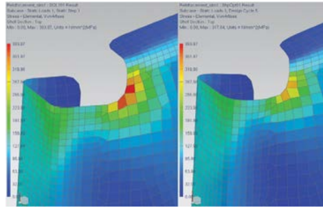
Left: Original design with high stress concentration. Right: New design after shape optimization.
