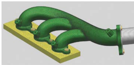
Model bolt preloading on solid elements such as for the bolts mounting this manifold assembly.
