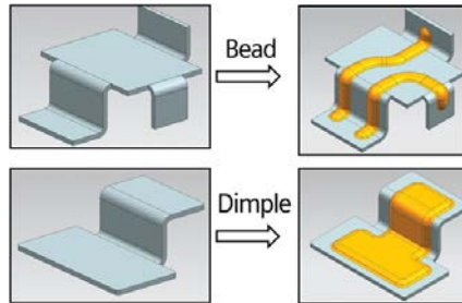
Beads and dimples can now be added after bends.
